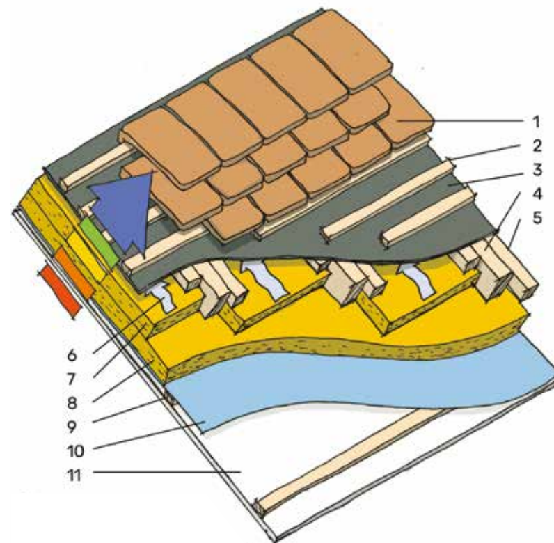
Skeiling insulation detail
