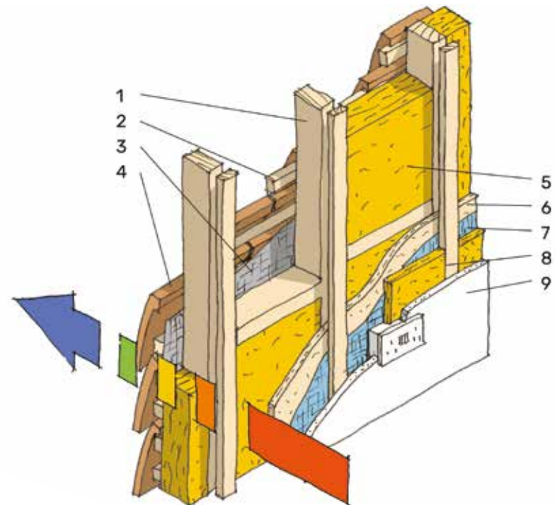
Traditional timber framed wall with insulation (after)
