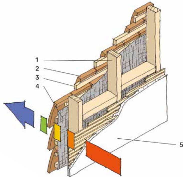
Traditional timber frame construction (before)
